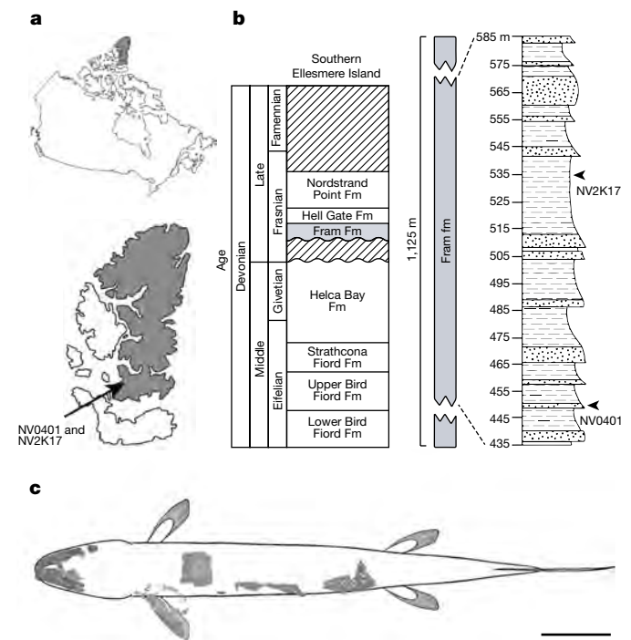
Fig. 1 | Locality and holotype of Qikiqtania wakei gen. et sp. nov. a , Specimen NUFV 137 was discovered on southern Ellesmere Island, Nunavut, Canada. b , The site, NV0401, lies 80 m below NV2K17, the site where T. roseae was discovered. c , Materials were \mu CT scanned and are shown here in dorsal aspect. General body shape based on specimen MHNM 06-2067 of E. watsoni 9 . Scale bar, 10 cm. Abbreviations: Fm, formation.
